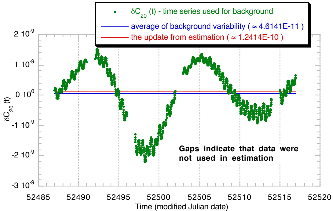
Figure 2 Depiction of the background model and its update from a GRACE solution.
