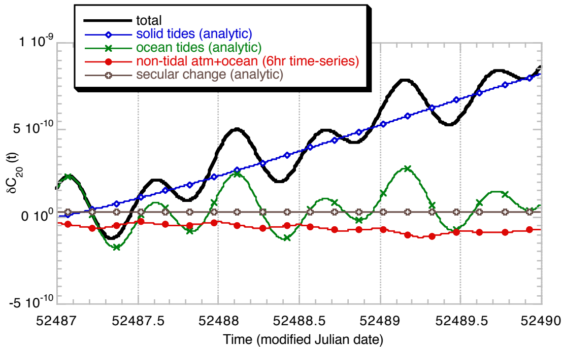
Figure 1 Components of the background model contributions to the C20 harmonic.
